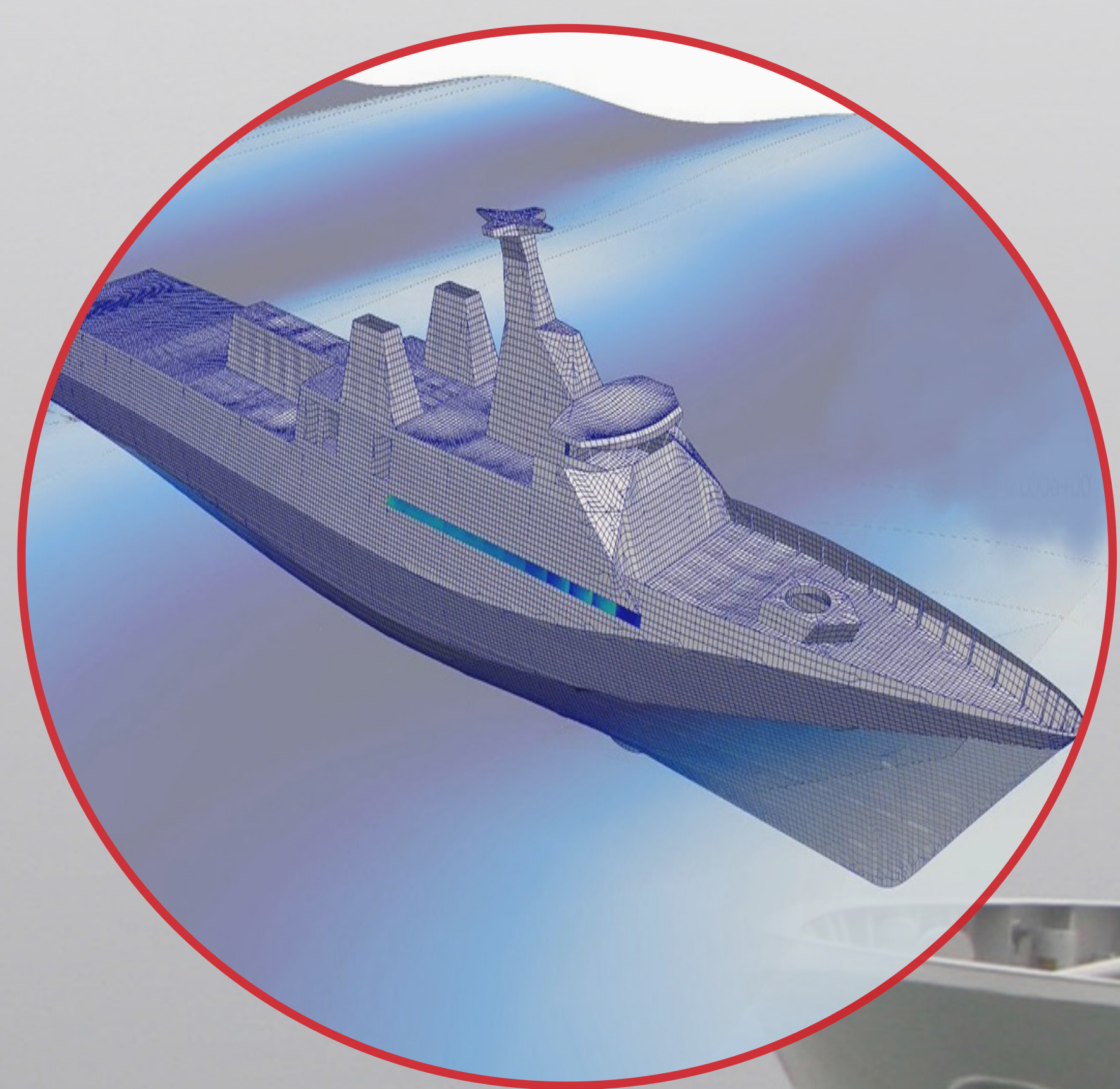
Ship motion fatigue load
