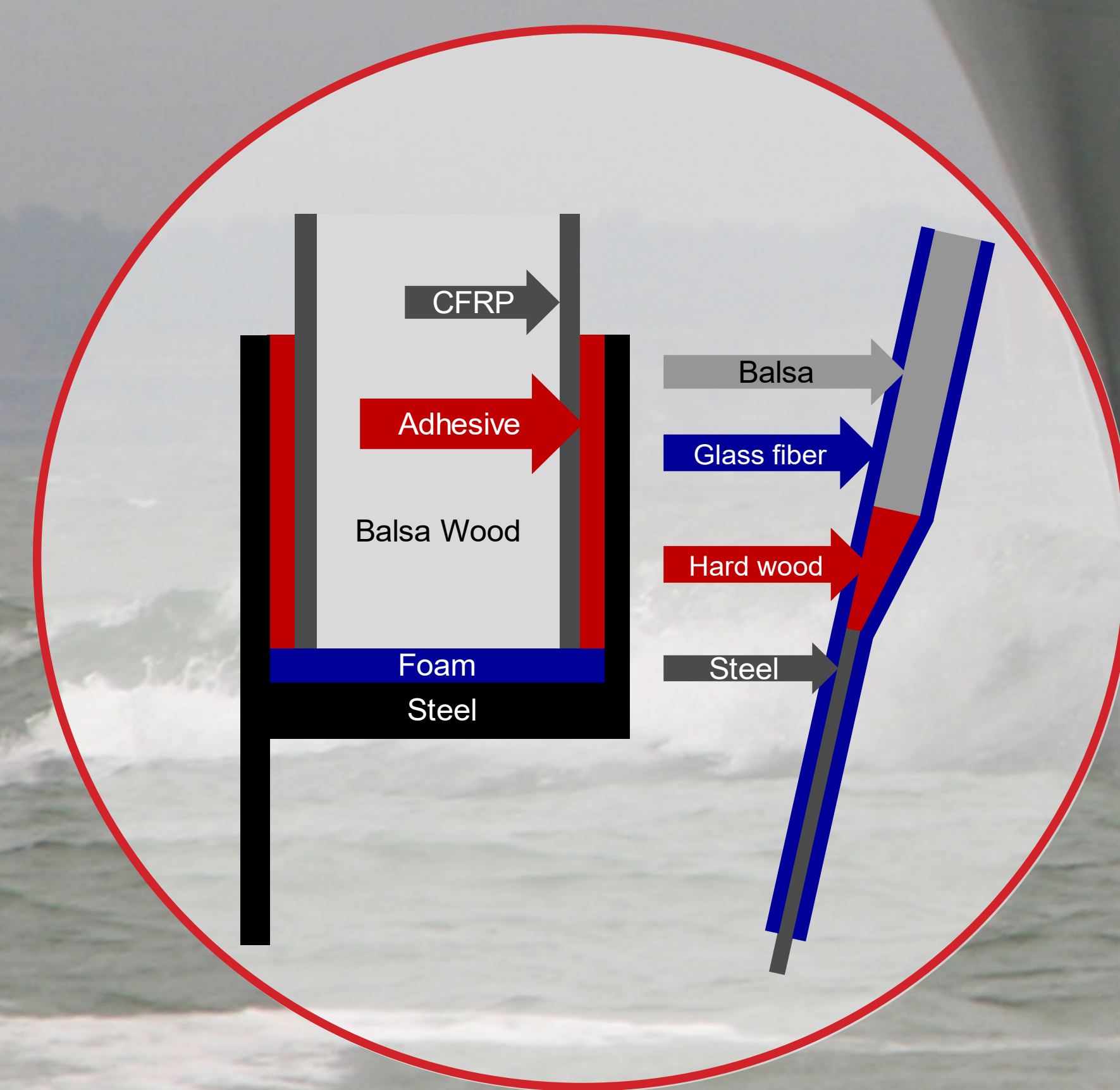
Two hybrid joint designs
